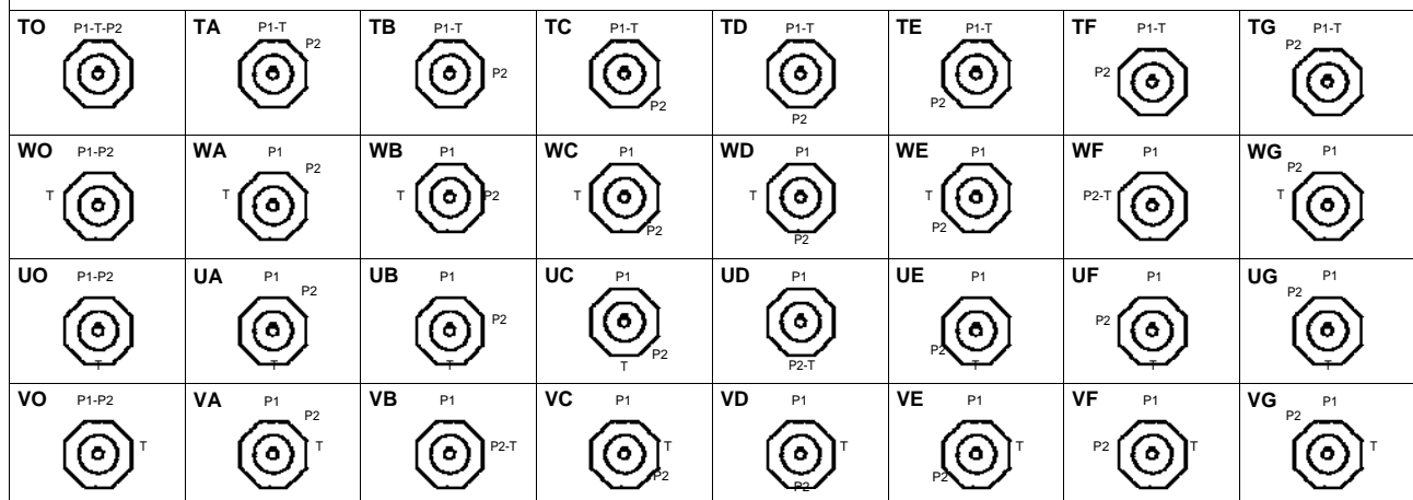
P1 = outlet port of first element; P2 = outlet port of second element; T = inlet port
